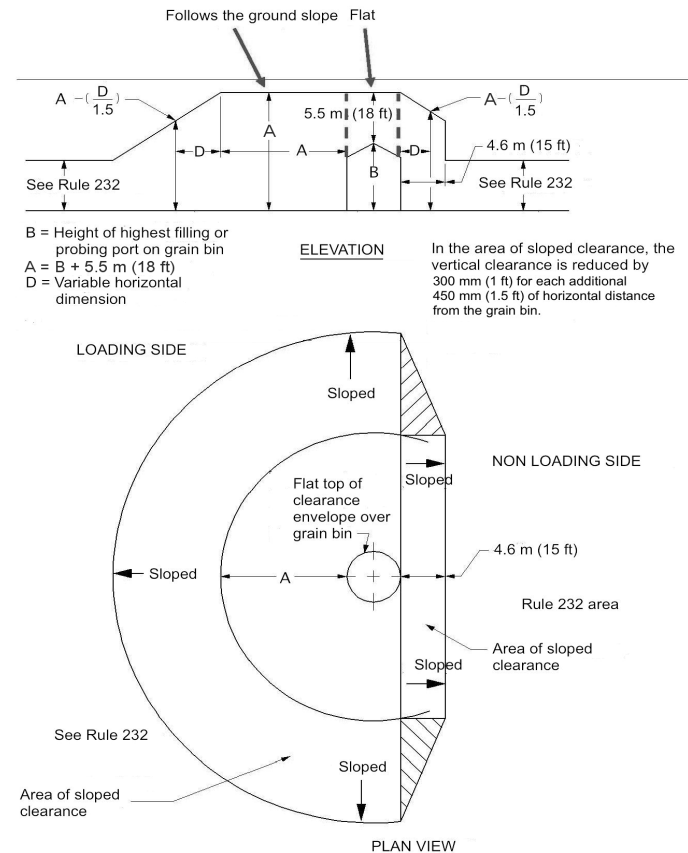
Figs. 232-4(b) Clearance Envelope for Grain Bins Filled by Portable Augers, Conveyors, or Elevators
